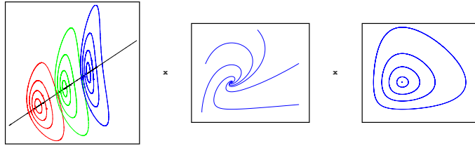
Figure 9: Representation of the system's dynamics associated to the graph T_4(T_6(G)) .
