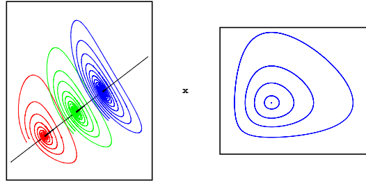
Figure 5: Representation of the dynamic of the system E_1 .
