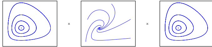
Figure 11: Representation of the system's dynamics associated to the graph T_1(T_4(T_6(G))) .
