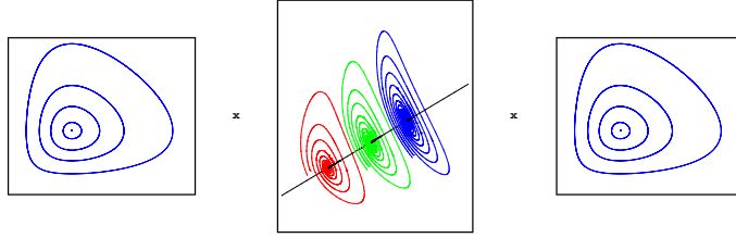
Figure 7: Representation of the system's dynamics associated to the graph T_3(T_6(G)) .
