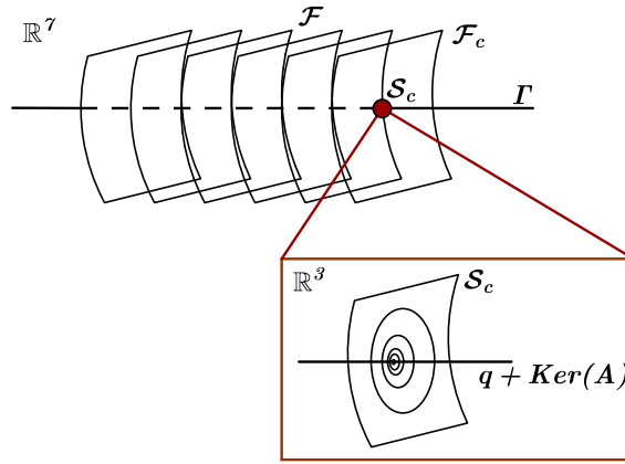
Figure 3: Phase portrait of a system E .
